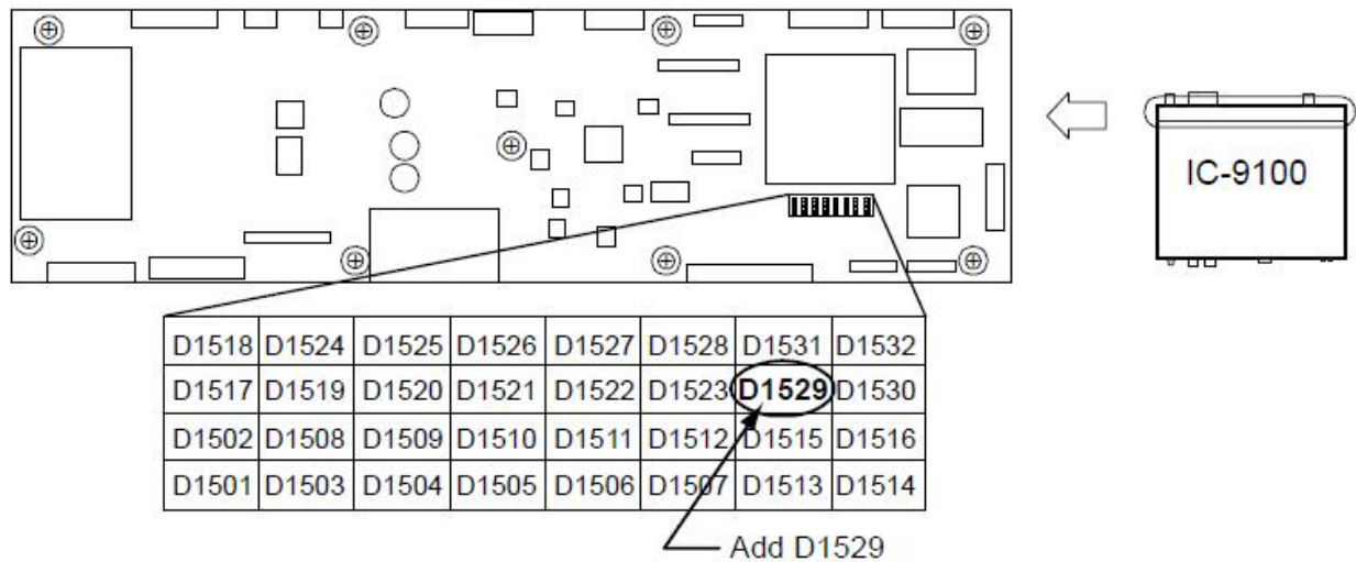
MAIN unit (top side)
